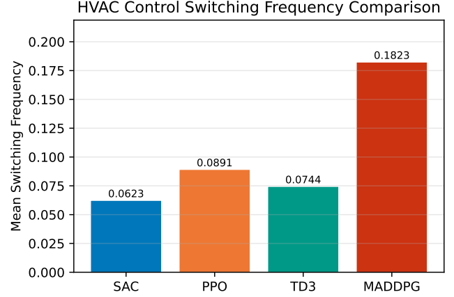
Figure 2. HVAC control switching frequency per algorithm. Lower values indicate smoother policies that reduce compressor wear. MADDPG’s frequency is computed across all five zone agents.
