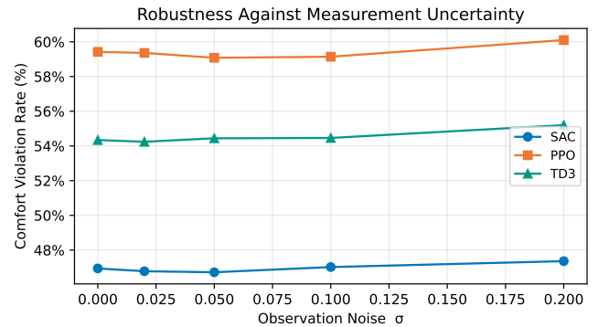
Figure 5. Comfort-violation rate as a function of measurement noise ( \sigma ). SAC degrades most slowly, demonstrating the implicit robustness conferred by entropy-regularised exploration.
