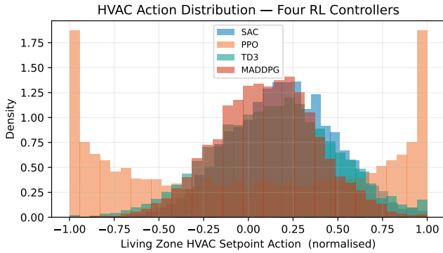
Figure 3. HVAC action distribution (Living zone) for all four controllers. SAC concentrates mass near moderate setpoints; PPO exhibits bimodal behaviour (near fully-on / fully-off).
